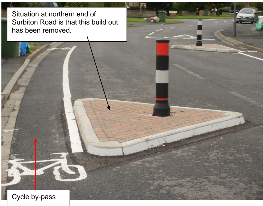
PINCH POINT WITH CYCLE BYPASSES. (1:100)
