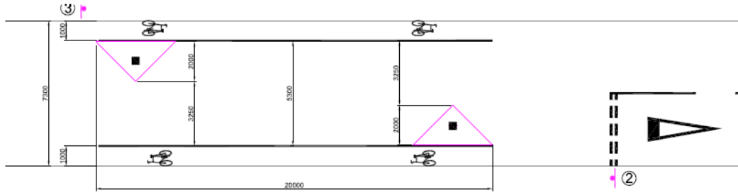
ONE WAY WORKING CHICANE WITH CYCLE BYPASSES. (1:100)
